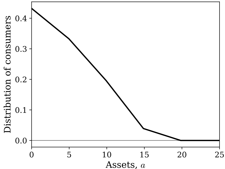
B. Simulated stationary distribution of assets
