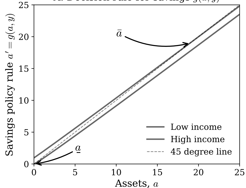
A. Decision rule for savings g(a, y)
