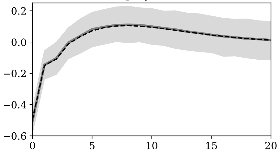
Local projection (LP)
