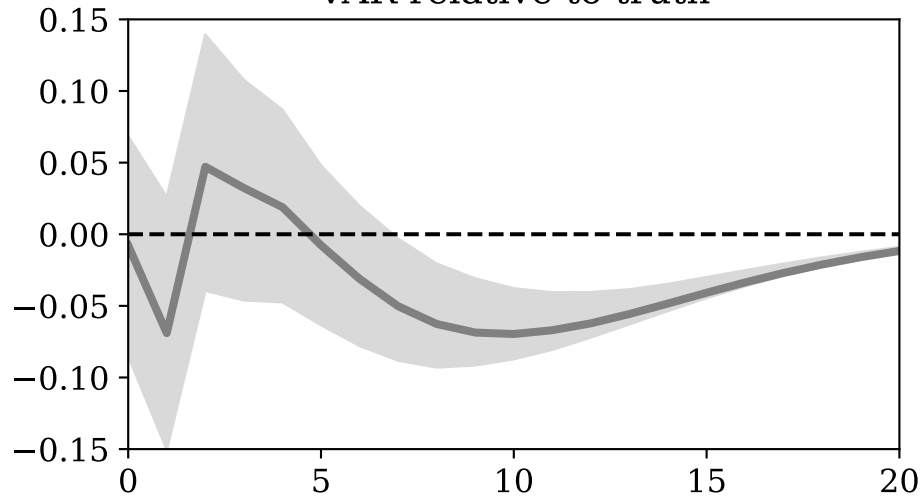
VAR relative to truth
