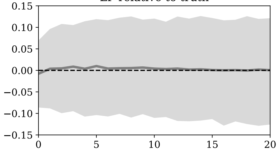
LP relative to truth
