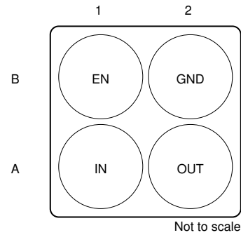
Figure 4-2. YCJ and YCK Packages, 4-Pin DSBGA (Bottom View)
