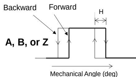
Figure 37: Incremental Output Hysteresis
