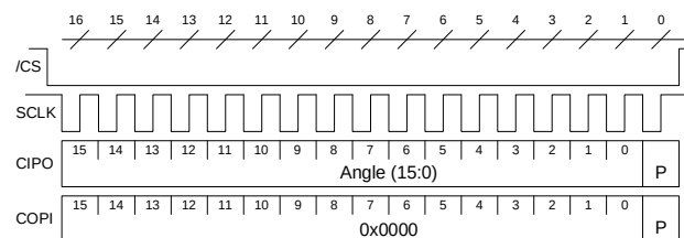
Figure 18: SPI Read Angle When an SPI Parity Check is Enabled
