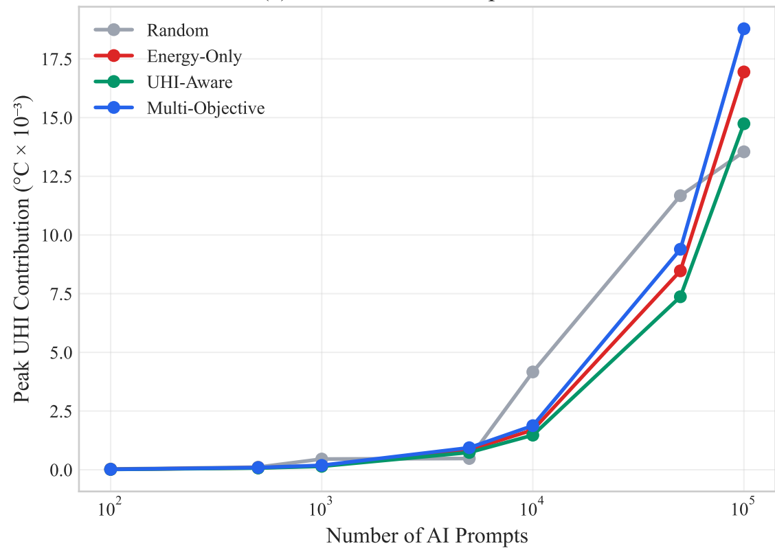
(a) Peak UHI vs Prompt Volume
