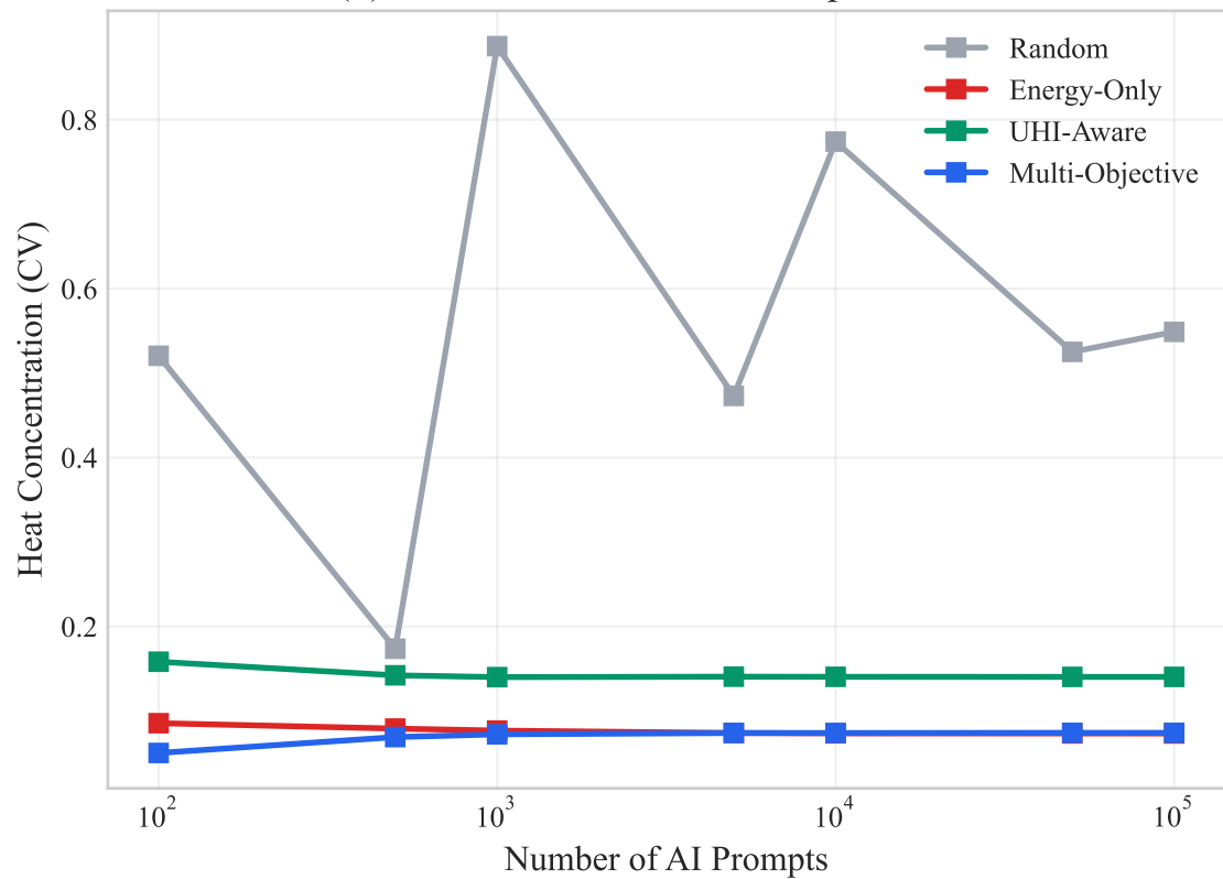
(b) Heat Distribution vs Prompt Volume
