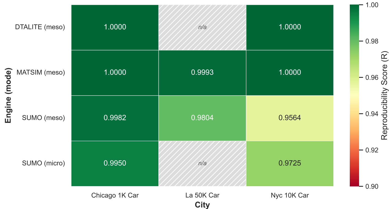
Figure 5.2: Reproducibility Analysis ( R = 1 - CV ; grey = not run)
