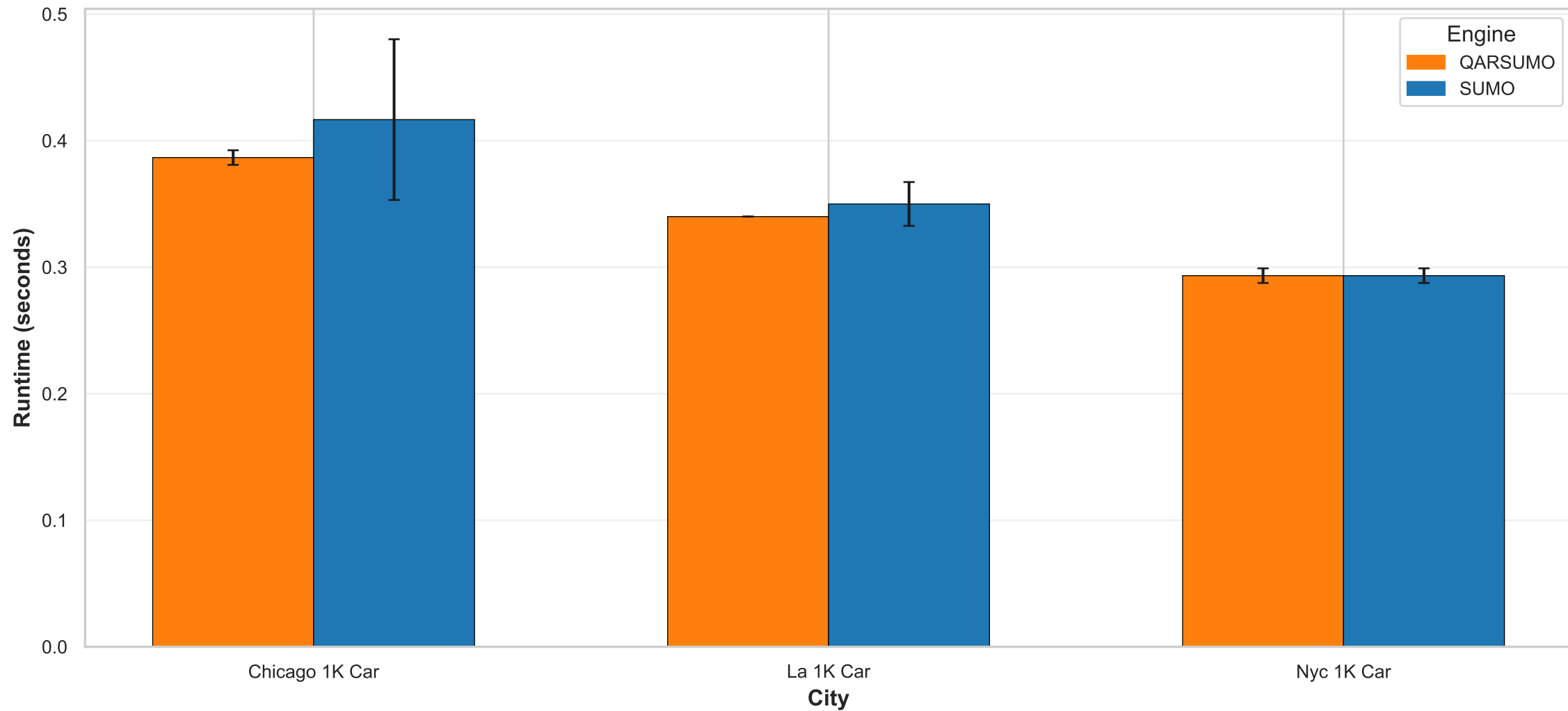
Figure 5.1: Runtime Comparison by City and Engine
