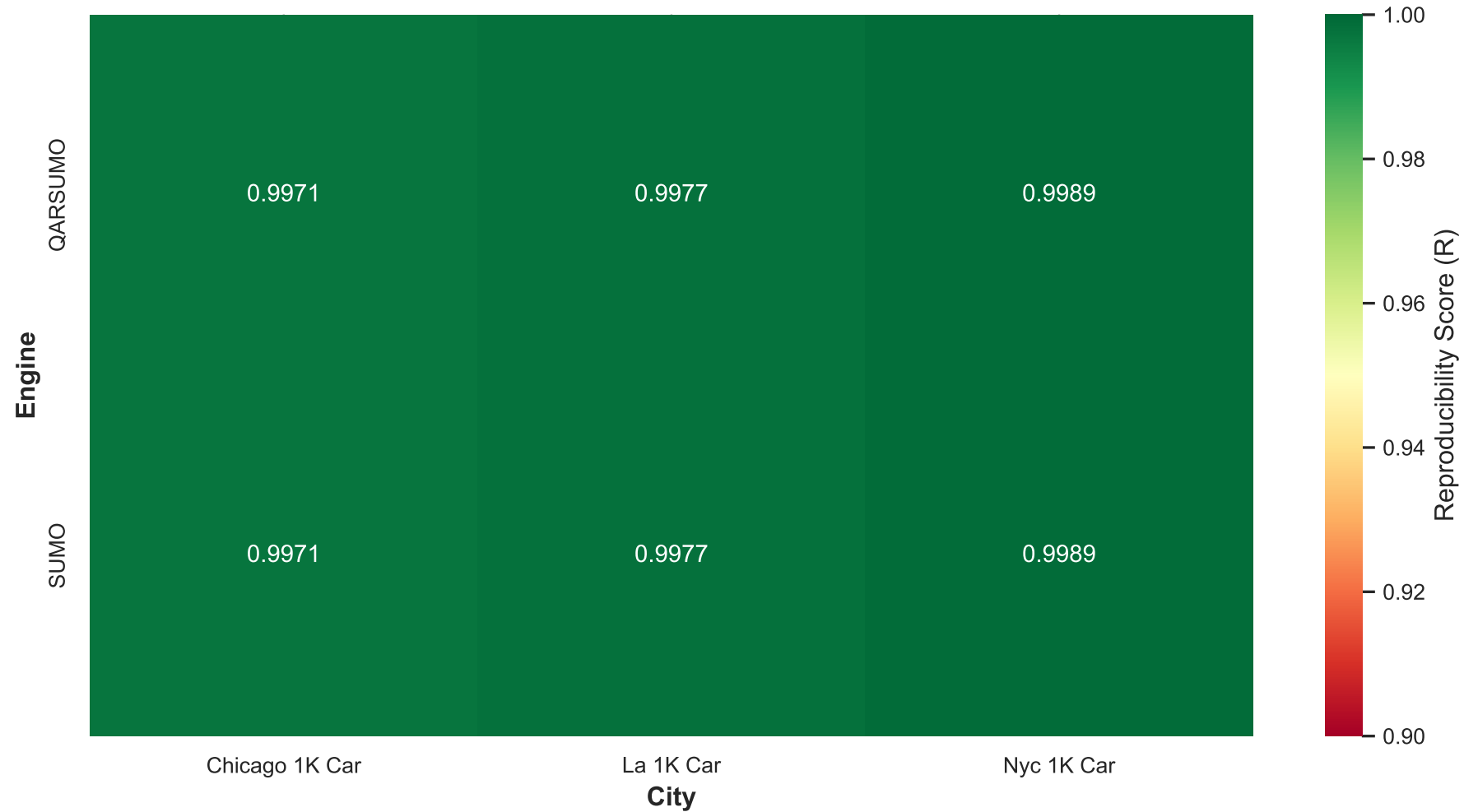
Figure 5.2: Reproducibility Analysis ( R = 1 - CV , higher is better)
