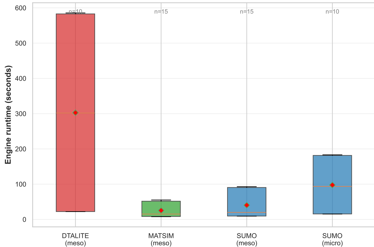
Figure 5.6: Engine Runtime Variability by Engine × Mode (engine subprocess only; box = IQR, diamond = mean, line = median)
