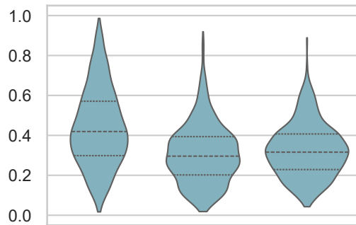
Control flow
