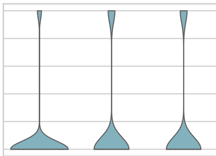
Operators
