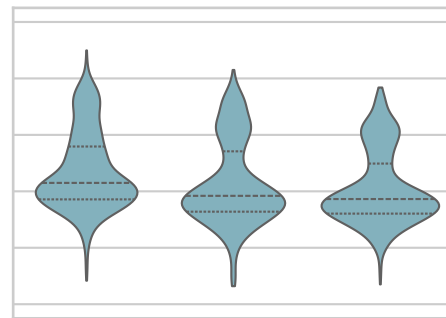
Identifiers
