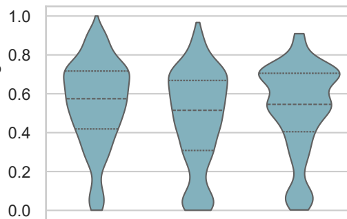
Data flow
