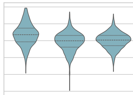
Complexity
