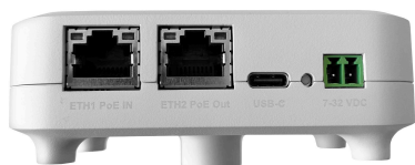
Figure 2: Connectors view of the device
