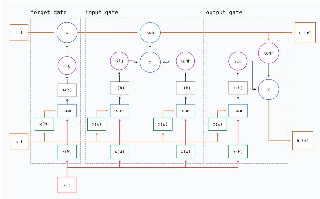
Gambar 3.2 Diagram Cell LSTM.
