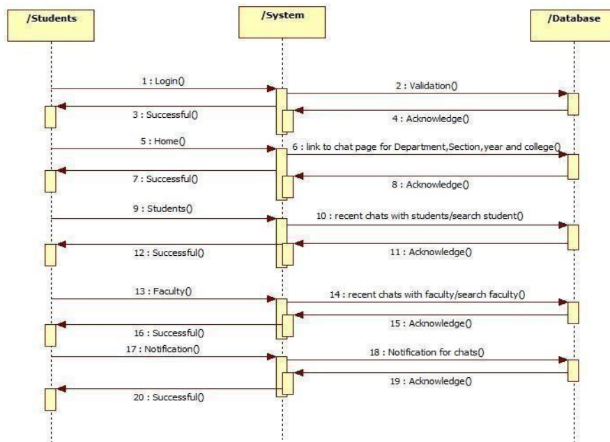
Fig. Sequence Diagram of Student
