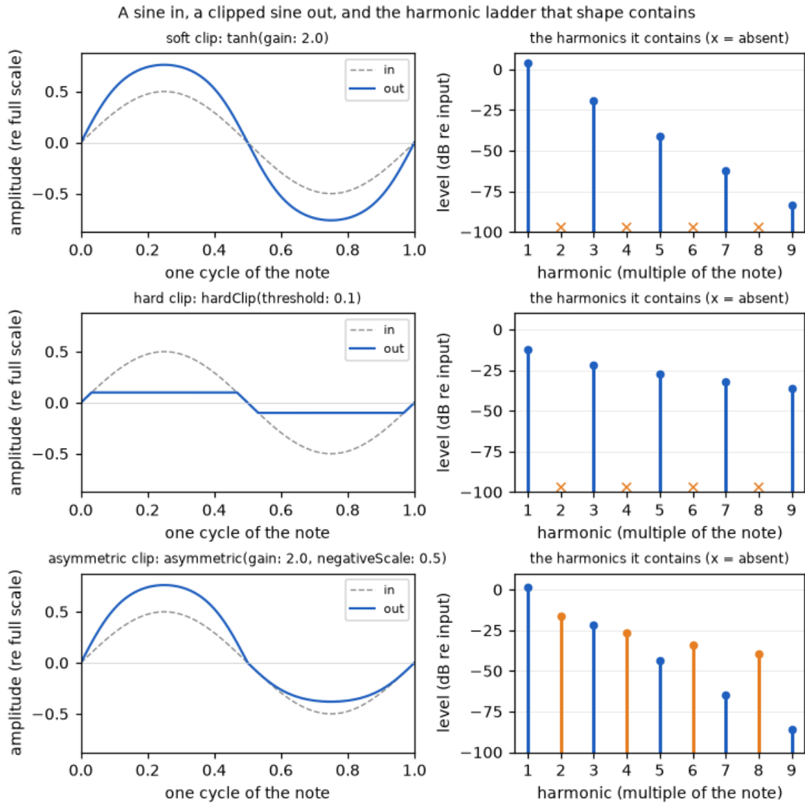
Figure 1: Three clippers, computed from their formulas at the amplitude the worked example uses (0.5 of full scale). Left: one cycle of a sine in (gray, dashed) and what comes out (blue). Right: the exact harmonic content of the output, in decibels relative to the input — each step of 20 down is a tenth of the size. Odd harmonics in blue, even in orange; a cross marks a harmonic that is exactly absent.
