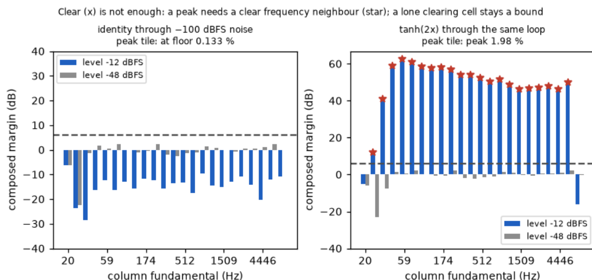
Figure 25: The corroboration rule. Each panel shows the composed margin at every column for the loudest rung (blue) and the quietest (gray) against the minimum (dashed); a cross marks a square that clears on its own, a star one whose neighboring note clears too. Left: a plain wire through a little noise — nothing clears, and the tile is a bound. Right: the soft clipper through the same loop — every clear square has a clear neighbor, and the tile is a peak.
