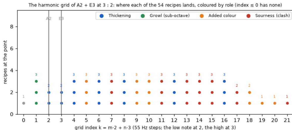
Figure 32: The harmonic grid of the requested fifth at its just ratio: every recipe at its grid step, stacked where several share a step and colored by the role assigned to that step; the two played notes marked. Step zero and below has no role.
