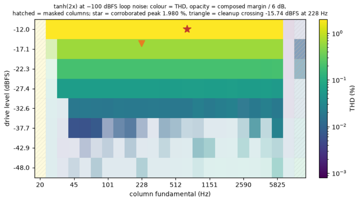
Figure 16: The worked example's map: the soft clipper on the hardware ladder through a loop with a little noise. Colour is THD; a square is drawn fainter the less clearly it stands above the floor described in the next section; the two fade columns are hatched; the star is the peak the tile quotes and the triangle is where the cleanup reading places the crossing at the tile's note.
