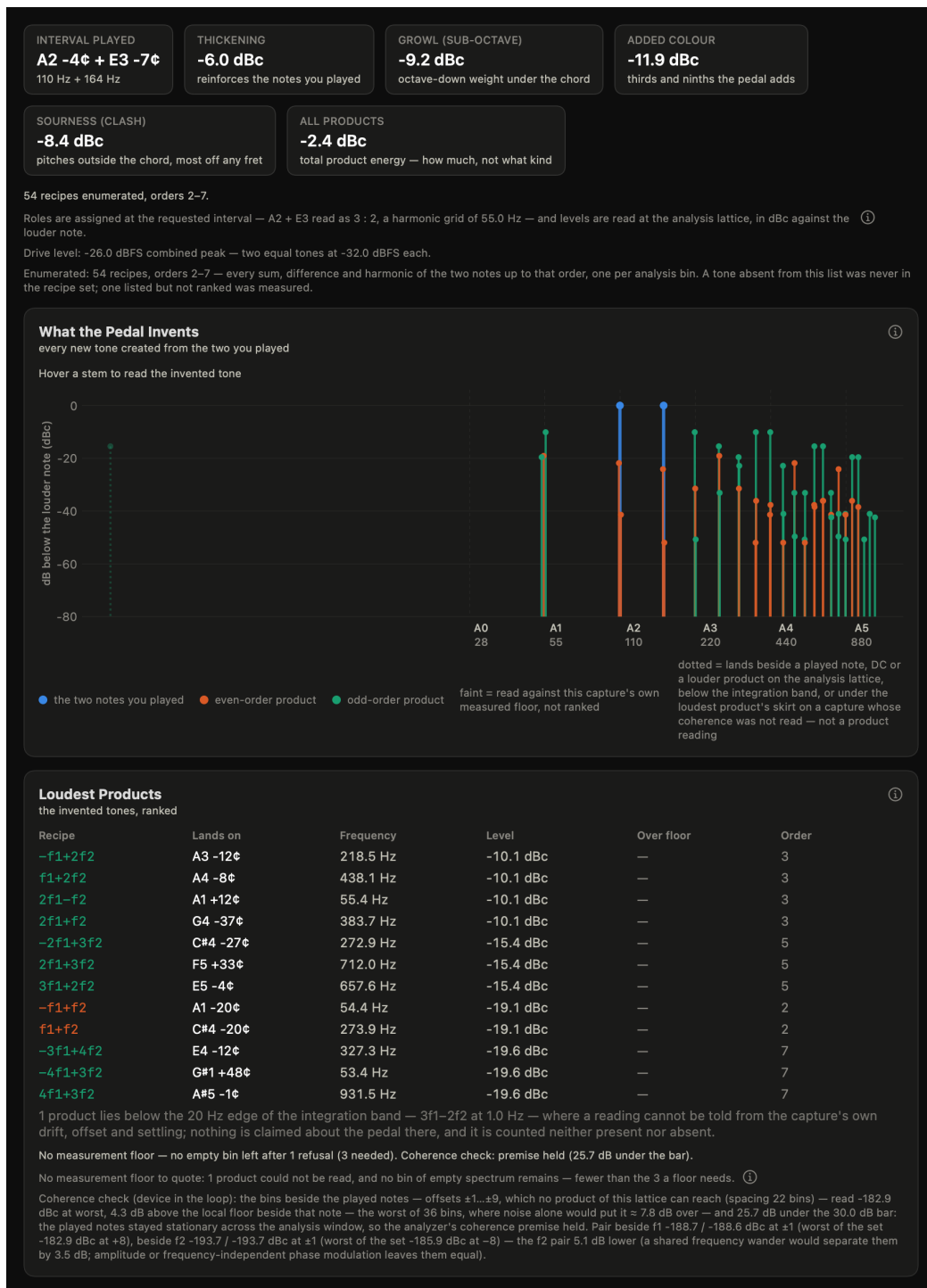
Figure 28: The Chord Roughness view as the app draws it, for its simulated pedal fed the default fifth at the standard drive.
