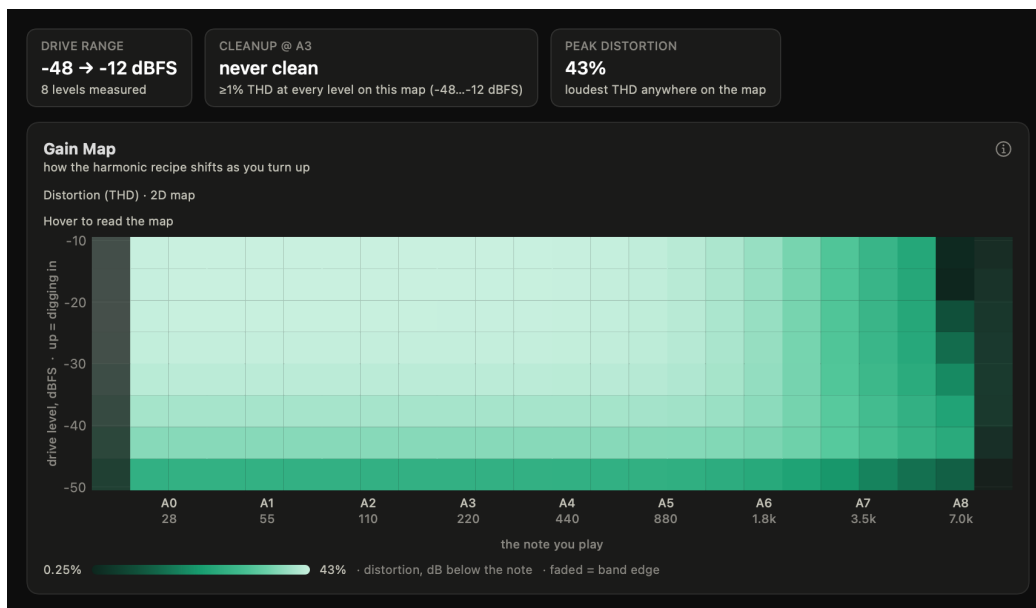
Figure 21: The Gain Map view as the app draws it, for its simulated pedal: the three tiles, the THD map over note and drive level, and the outermost columns drawn faded.
