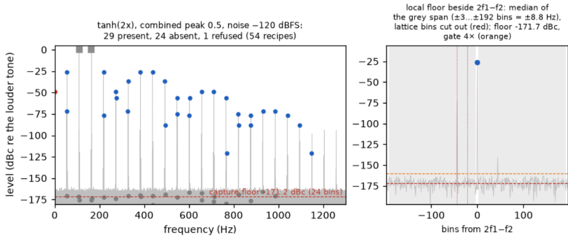
Figure 27: The worked example, a soft clipper at the loudest hardware drive on the shipped fifth through seeded noise. Left: the spectrum with every recipe marked measured (blue), nothing found (grey) or refused (red), the two notes as squares, and the capture floor as the dashed rule. Right: the local-floor neighbourhood of one recipe, with the lattice slots cut out (red), the floor (red, dashed) and the gate (orange, dashed).
