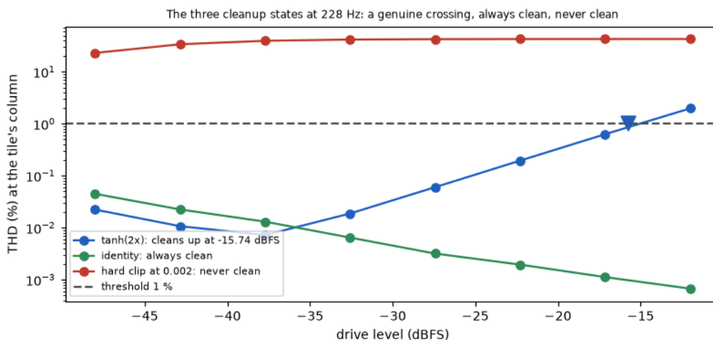
Figure 20: THD against loudness at the tile’s column for the three cleanup states: the soft clipper crosses the line between two rungs (the triangle marks the crossing); a plain wire stays under it throughout; a hard clipper is over it at every rung.
