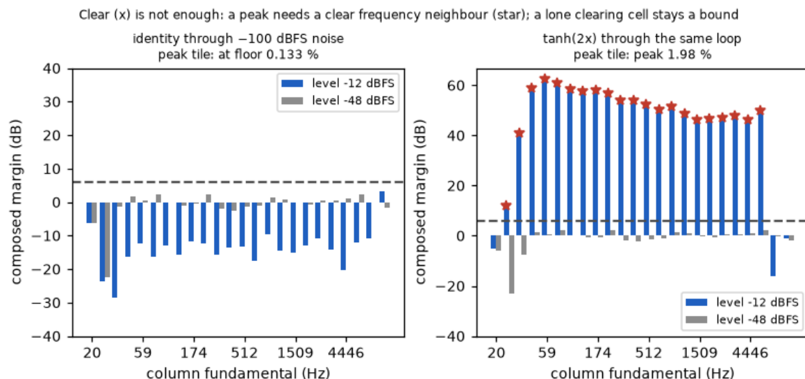
Figure 19: The corroboration rule. Each panel shows the composed margin at every column for the loudest rung (blue) and the quietest (grey) against the minimum (dashed); a cross marks a square that clears on its own, a star one whose neighbouring note clears too. Left: a plain wire through a little noise — nothing clears, and the tile is a bound. Right: the soft clipper through the same loop — every clear square has a clear neighbour, and the tile is a peak.
