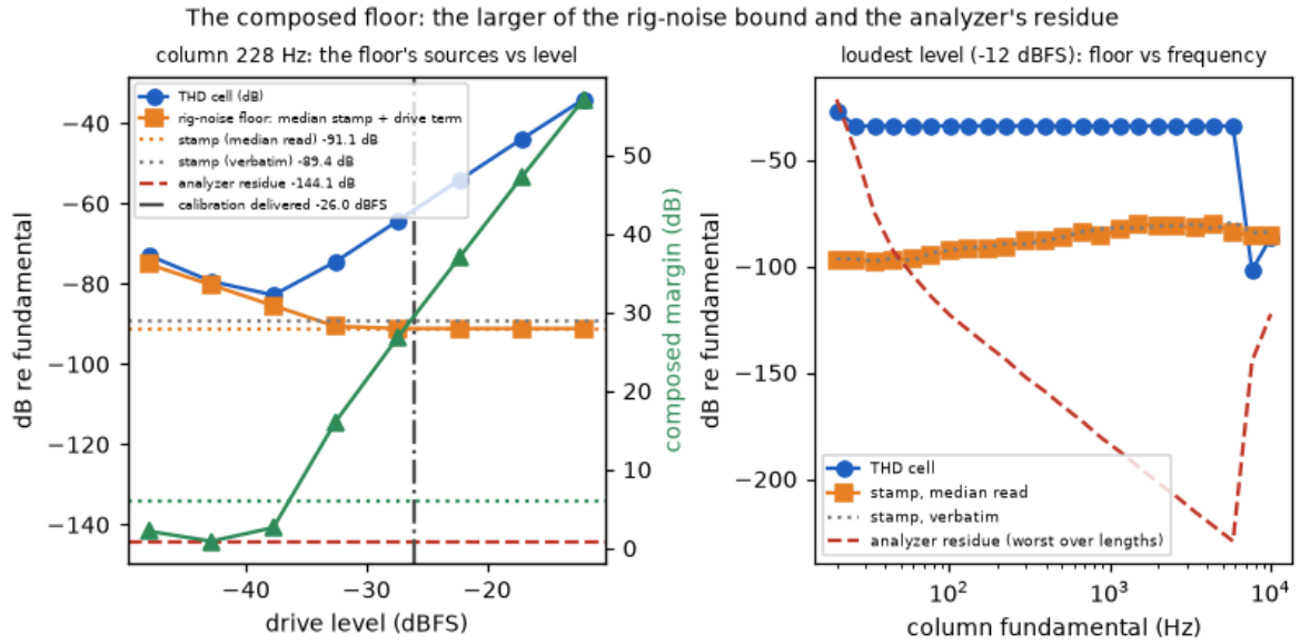
Figure 18: The floor, composed from its sources, at one column of the worked example (left): the square’s THD against loudness, the calibration’s floor read verbatim and through the median, the drive term rising below the calibration’s own level and flat above it, the analysis’s residue, and the margin (green, right-hand scale) against its minimum. Right: the same at the loudest rung against note.
