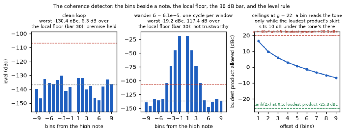
Figure 25: The coherence check. Left: the nine slots either side of the high note on a clean loop through a little noise, with the local floor beside the note (grey) and the bar above it (red) — within a few decibels of the floor, premise held. Middle: the same slots on the pipeline’s wander fixture, a shared drift of both notes at one cycle per window — far over the bar, not trustworthy. Right: the ceiling each slot sets on the loudest invented tone at the shipped spacing, with the worked example’s loudest tone far below every ceiling and a squarer driven above its own notes clearing none.
