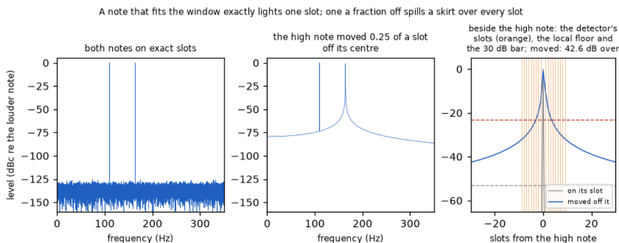
Figure 22: Two notes at the standard drive through a little noise, read through the analysis window the next chapter uses. Left: both notes on exact slots — two lines and a flat floor. Middle: the high note moved a quarter of a slot off its centre, as the panel’s title states; its skirt covers the whole span. Right: the slots either side of the high note in both cases, the nine the coherence check reads marked, with the local floor beside the note and the bar above it for the moved case.
