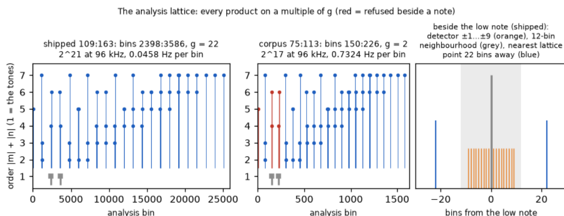
Figure 23: The analysis lattice. Left: every recipe as a stem at its slot and order on the shipped fifth, the two played notes as squares at order one; every stem sits on a multiple of the spacing. Middle: the same on the crowded probe every earlier record was made on — the four recipes two slots from the notes and the one two slots from zero are red, refused on position. Right: the slots beside the low note on the shipped lattice — the nine the coherence check reads, the neighbourhood the reading rule guards, and the nearest recipe a spacing away.
