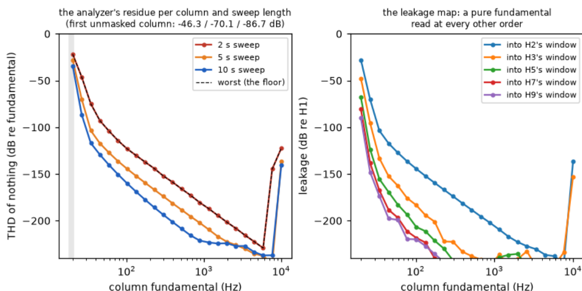
Figure 17: Left: the analysis's own residue at every column of the map for the three sweep lengths — the fade-in leak at the first unmasked column, largest on the shortest sweep — and the worst case the record assumes (dashed). Right: the leakage map used by the check described later: a signal containing only its note, read at every other harmonic.
