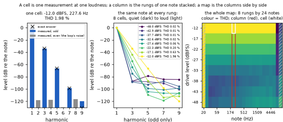
Figure 15: A map is a stack of single-loudness measurements. Left: one cell of the worked example — the soft clipper at the loudest rung of the hardware ladder, at the note the cleanup tile reads — as the measured level of each harmonic relative to the note (blue for the odd harmonics, grey for the even ones, which this clipper does not make and which read the loop’s own noise), with the exact answer marked by a cross; the ninth harmonic’s exact answer lies under the loop’s noise, just below the pane. Middle: the same note at all 8 rungs, quiet to loud, each rung’s THD in the legend. Right: the whole map, THD as colour, the fade columns hatched, the column outlined in red and the cell in white.
