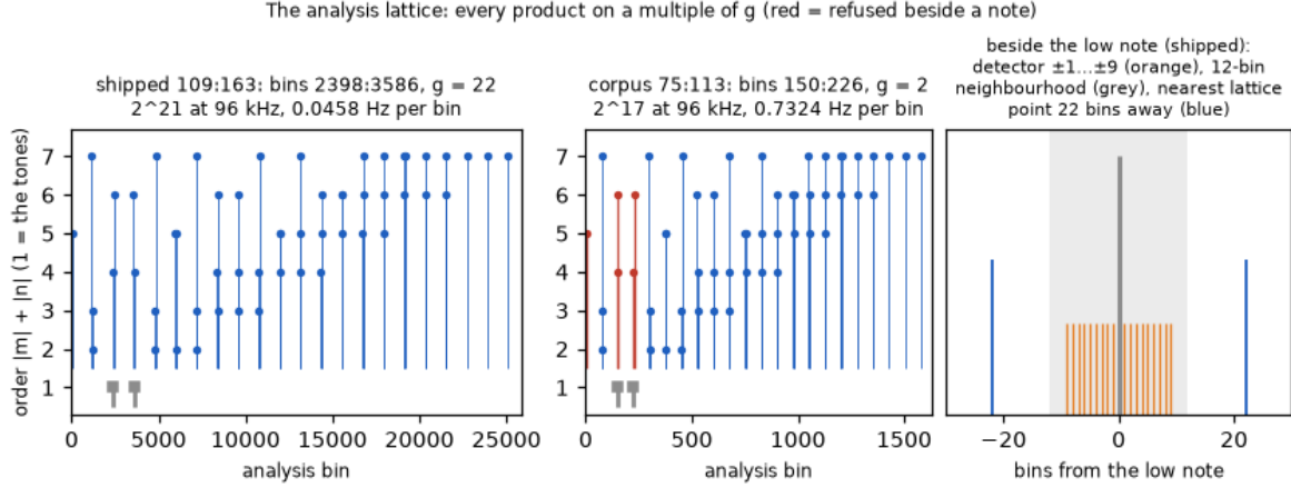
Figure 25: The analysis lattice: every enumerated recipe as a stem at its bin and order on the shipped fifth (left) and on the corpus probe every earlier record was captured on (middle), the two tones as squares at order one. On the corpus probe the four even-order recipes two bins from the played notes and the one two bins from DC draw red: refused on position (§7.4). Right: the bins beside the low note on the shipped lattice — the detector’s offsets, the played-tone neighbourhood, and the nearest lattice point a spacing away.
