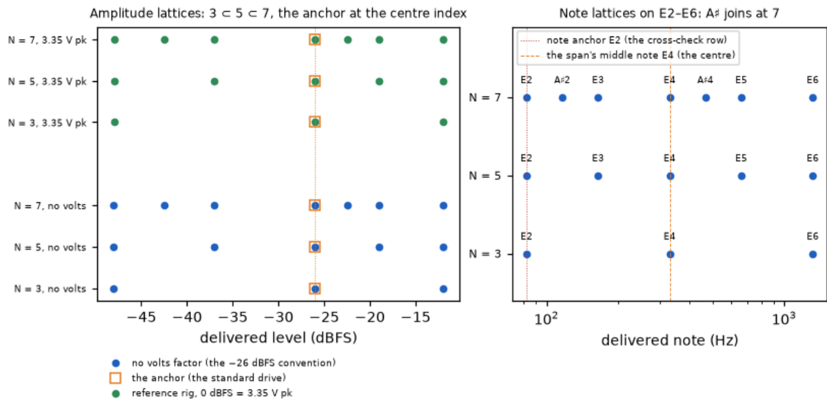
Figure 31: The two lattices at N = 3, 5, 7 . Left: the amplitude lattice on the no-volts convention and on the reference rig's factor (equal by construction), the anchor at the centre index of every dimension, the floor a fixed span below it, the ceiling fixed; every smaller lattice is a subset of the larger. Right: the note lattice on the default span, the octave ladder at 5 with A#2 and A#4 joining at 7; E2 (dotted) is the cross-check row and E4 (dashed) the centre — two different rows.
