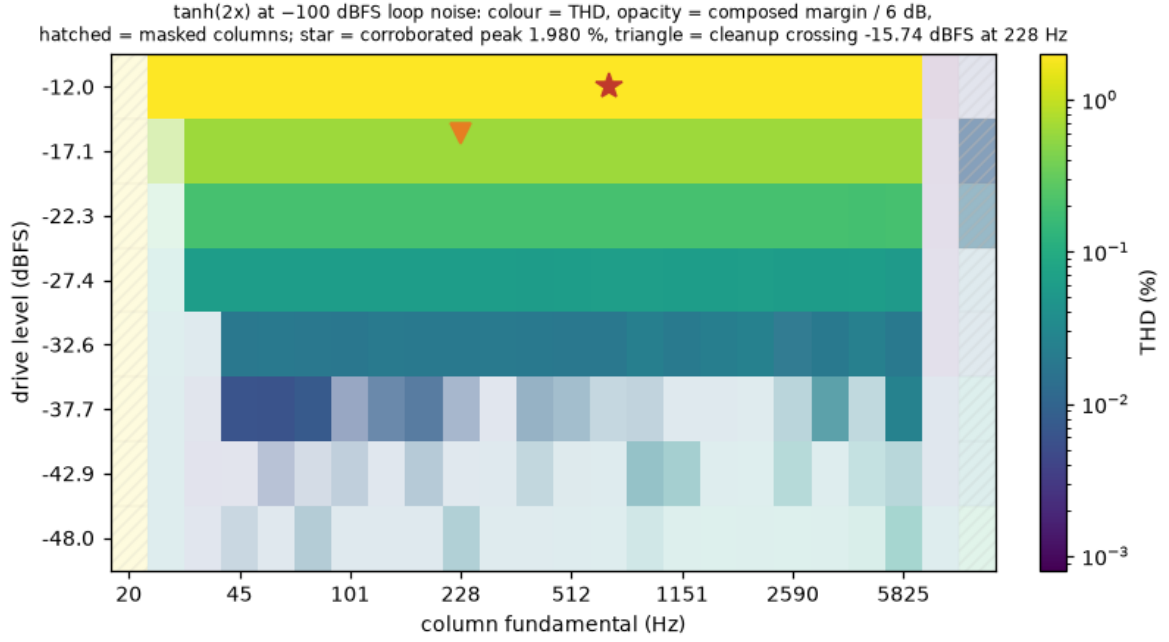
Figure 19: The worked example's map: y = \tanh(2x) on the hardware lattice through a loop with seeded noise, every cell coloured by its THD and drawn at an opacity that follows its composed margin, the two edge columns hatched, the corroborated peak starred and the cleanup crossing marked at the tile's column.
