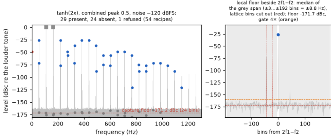
Figure 27: The worked example, y = \tanh(2x) at a combined peak of 0.5 on the shipped fifth through seeded noise: the analysed spectrum with every enumerated product marked present (blue), absent (grey) or refused (red), the two tones as squares, and the capture floor as the dashed rule (left). Right: the local-floor neighbourhood of one product, the median of the grey span with every lattice bin cut out, and the gate four times above it.
