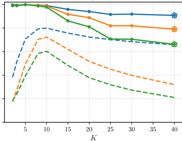
MNIST / UMAP
