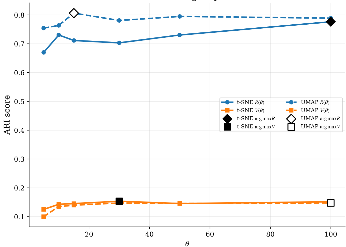
20 Newsgroups
