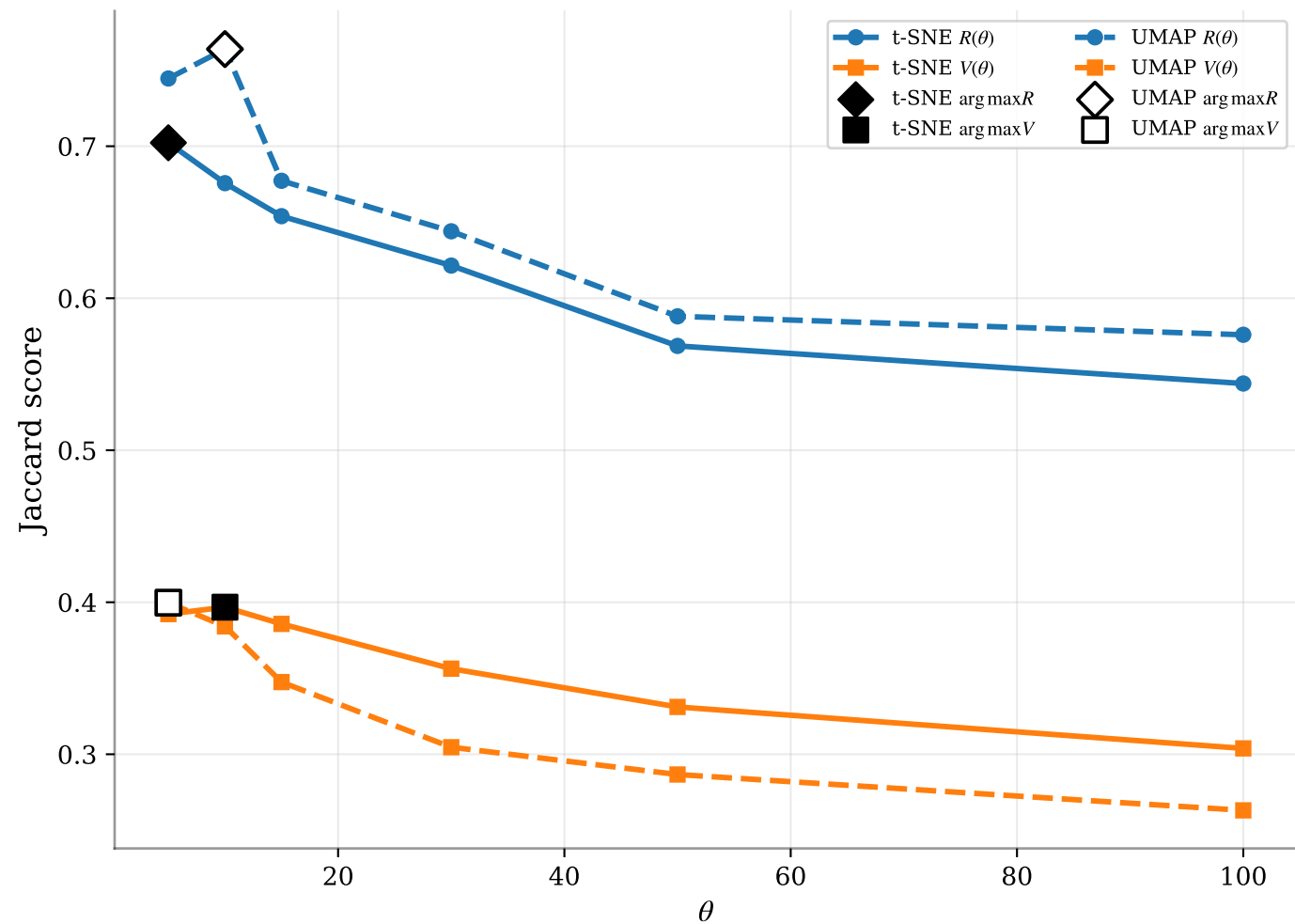
Olivetti Faces
