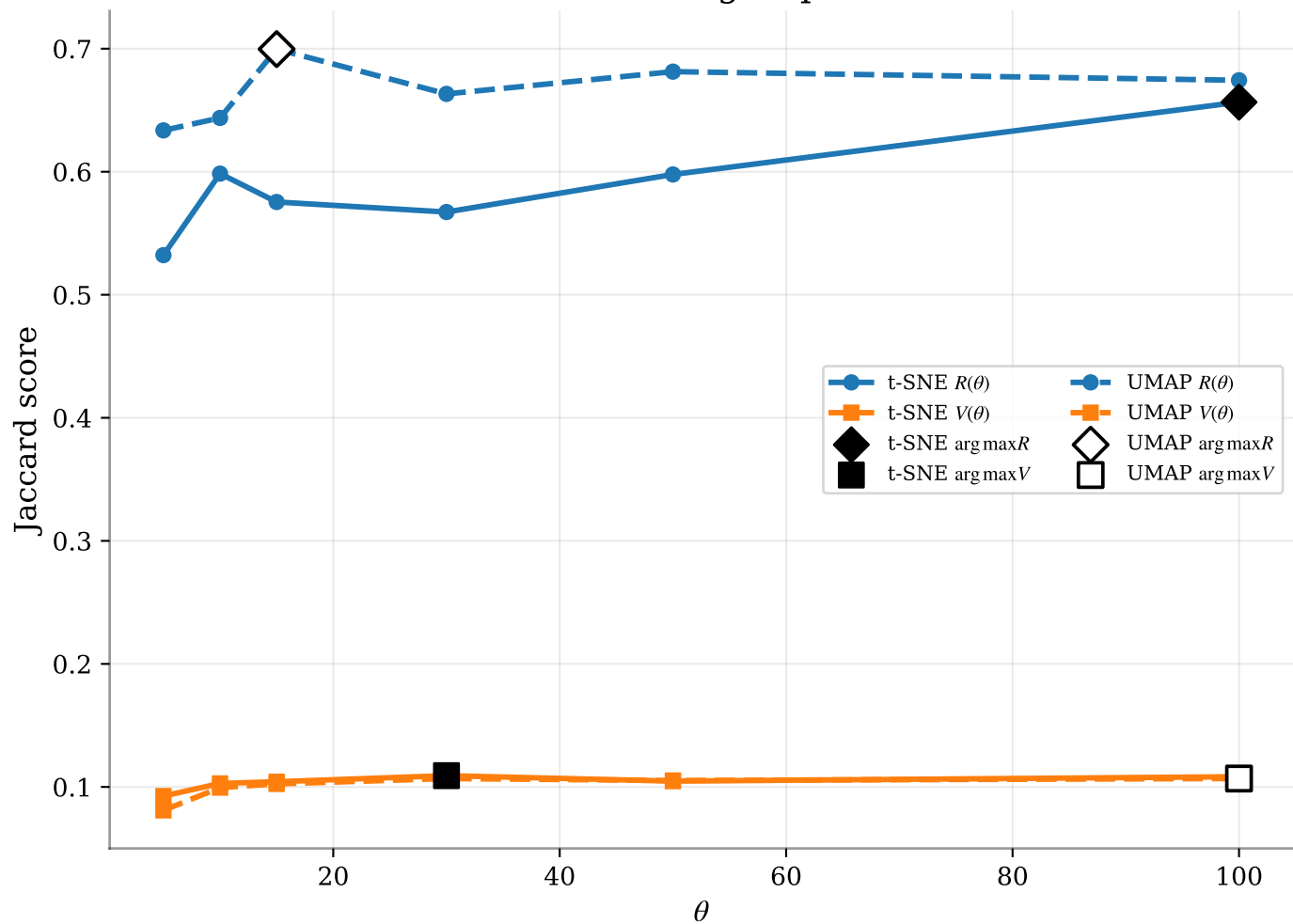
20 Newsgroups
