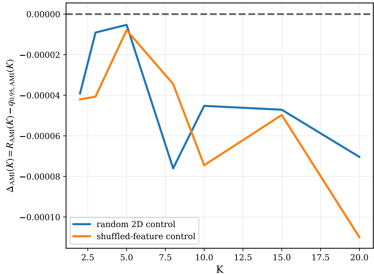
MNIST / UMAP
