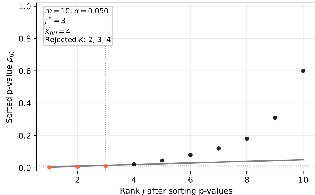
BH procedure on synthetic data
