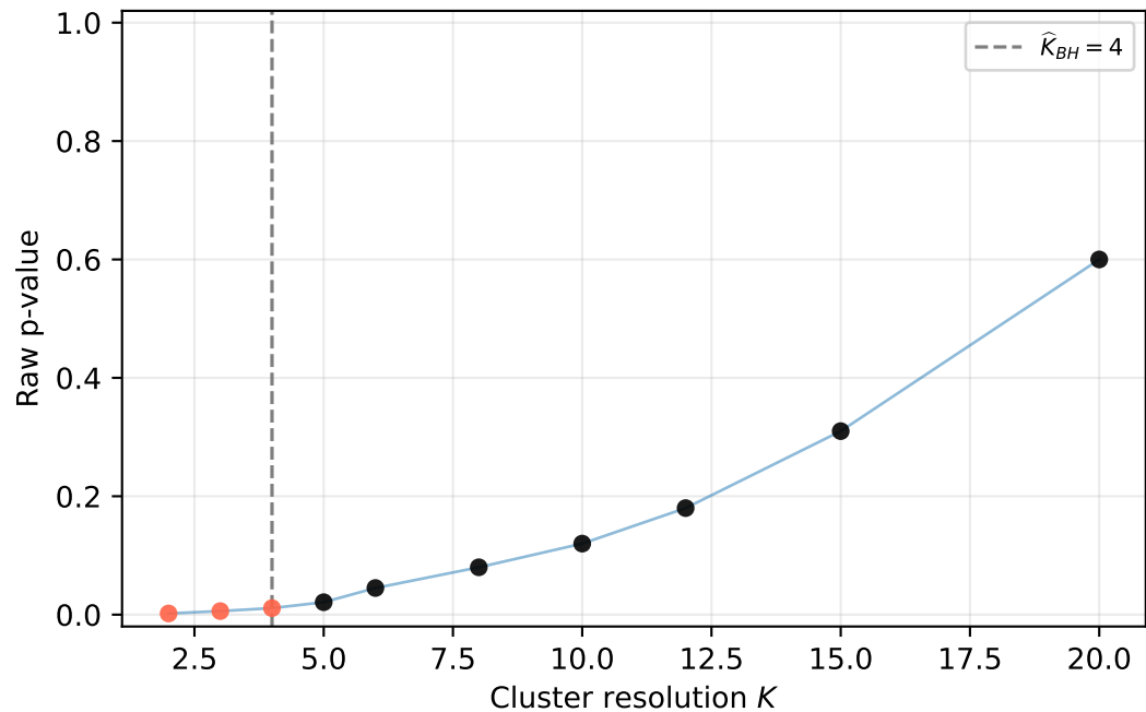
Synthetic p-values in K -space
