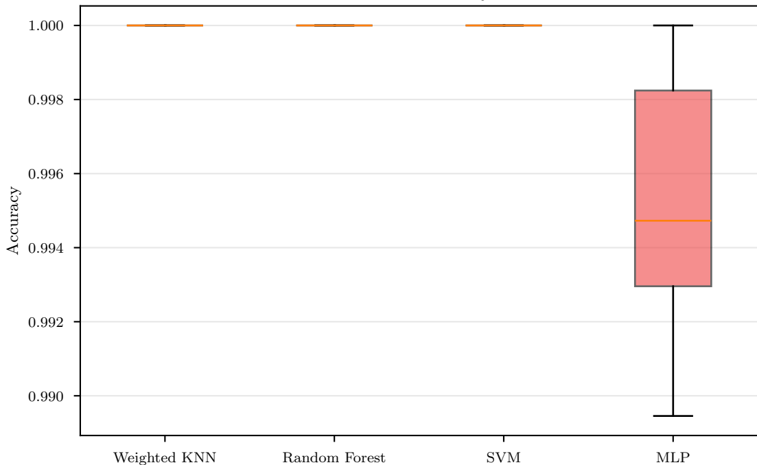
Cross-Validation Accuracy Distribution
