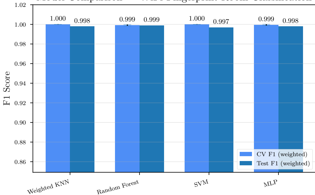
Model Comparison — WiFi Fingerprint Room Classification
