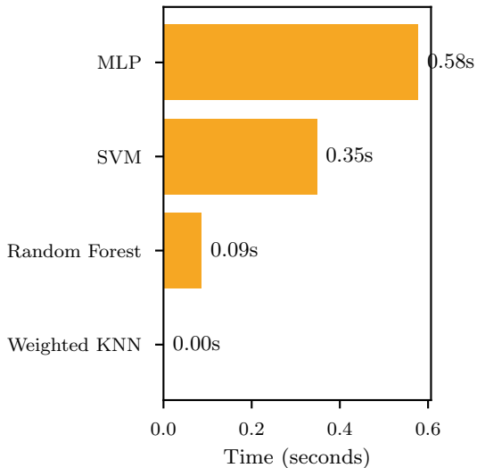
Training Time
