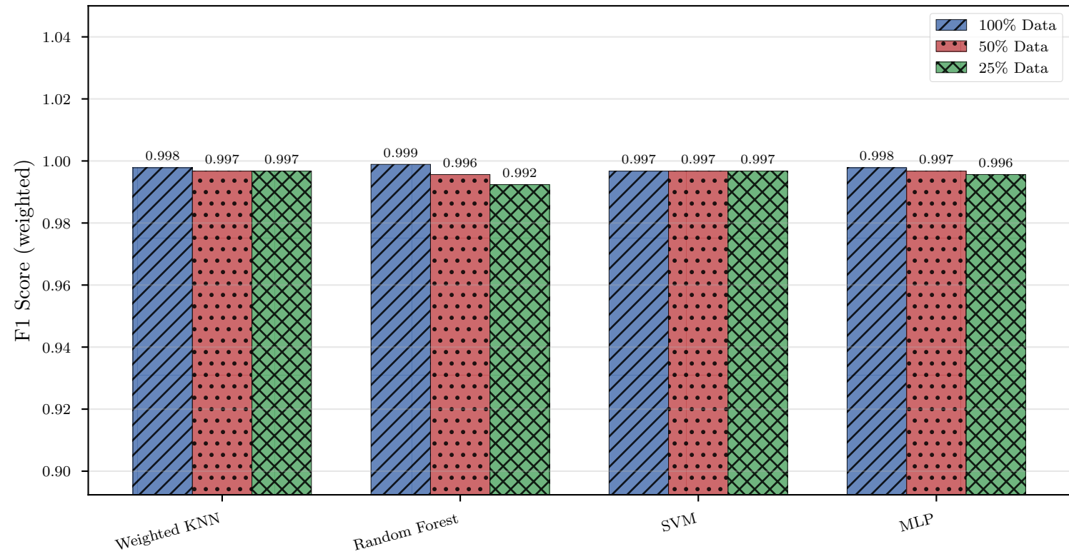
Impact of Training Data Reduction on Model Performance
