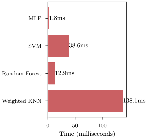
Prediction Time (full test set)
