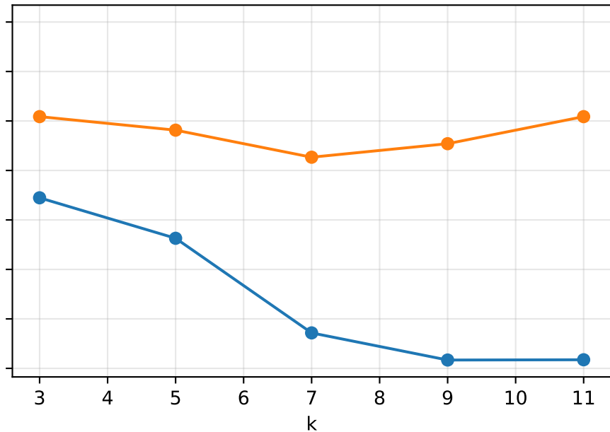
Euclidean Distance
