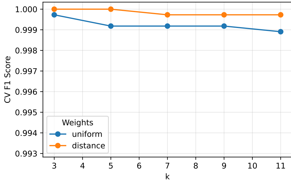
Manhattan Distance
