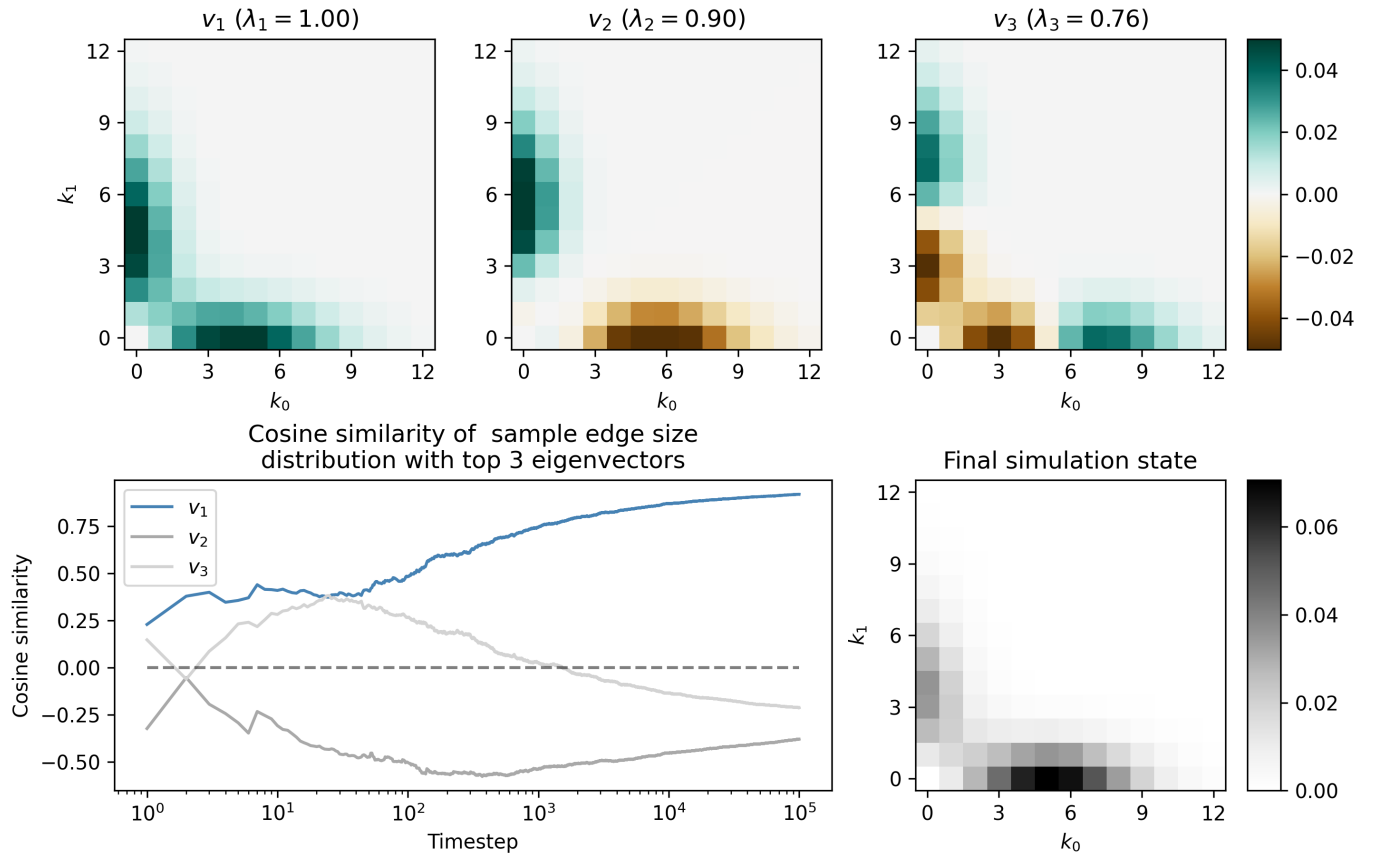
FIG. 1. Dynamics! Top shows the three leading eigenvectors of the distribution p(k_0, k_1) . Bottom left gives the cosine similarity (normalized projection) between one run of simulation dynamics and these eigenvectors. Bottom right gives the final simulation state.
