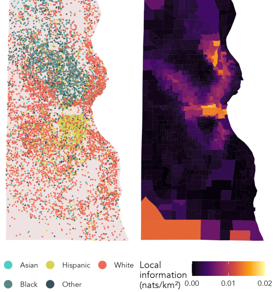
Figure 7: Local information in Milwaukee, Wisconsin. A smoothing kernel of bandwidth 1 km was applied to the original population data, and the local information was then computed at each block group using eq. (13) with local linear regression to estimate the spatial derivatives of \Upsilon . The map contains 10,000 dots corresponding equal units of population within each demographic category and block group.
