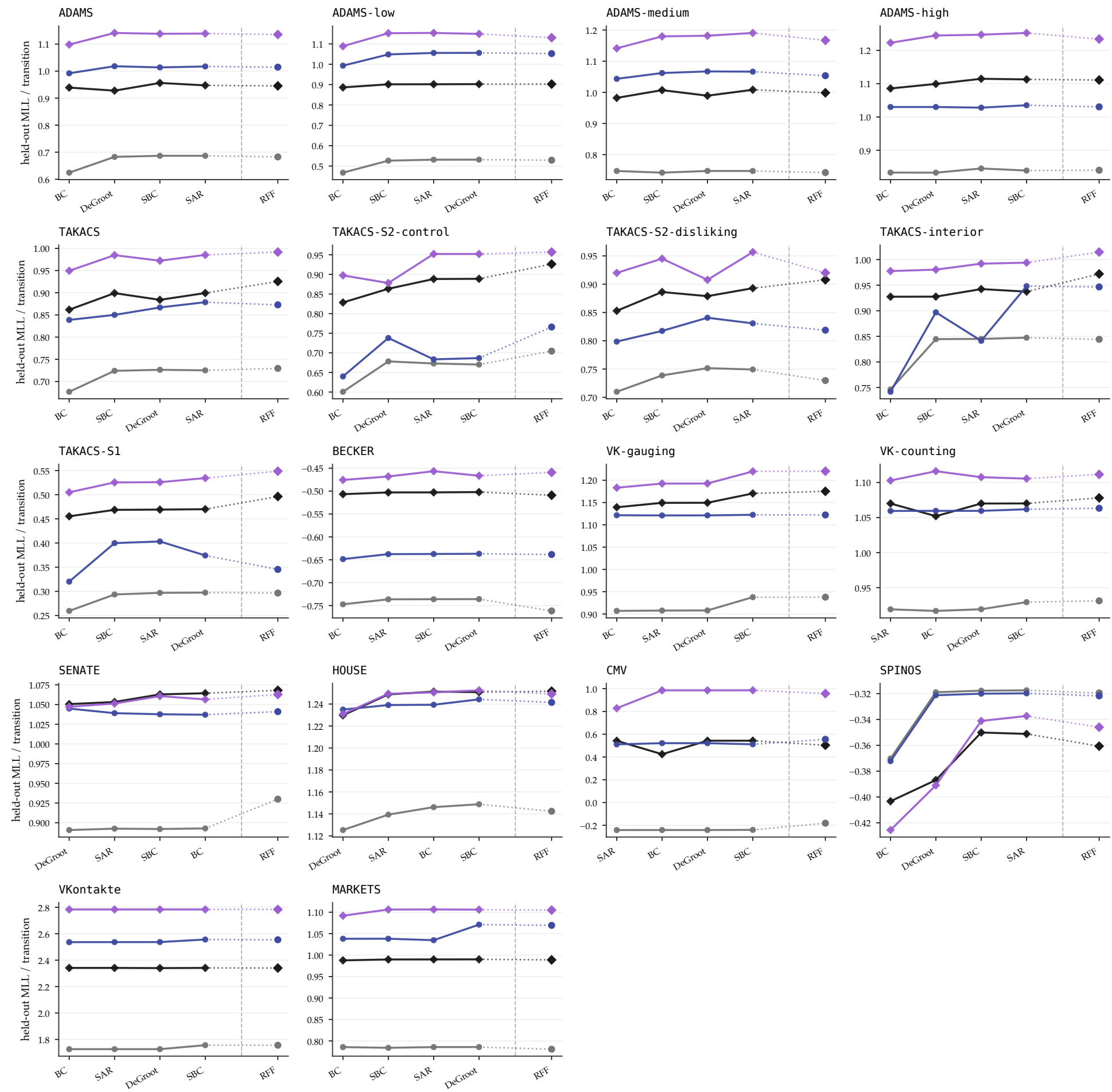
Kernel ordering within each noise family (pairwise)
