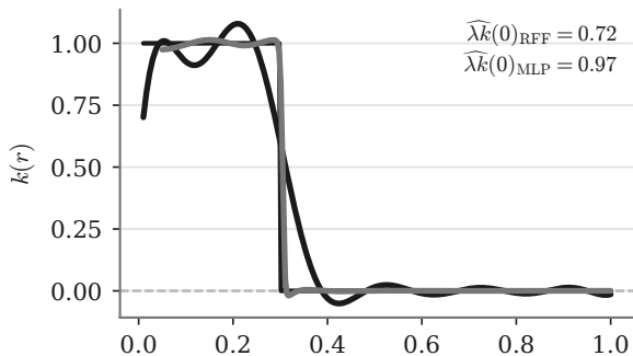
Bounded Confidence
