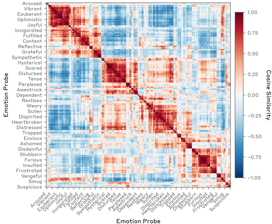
Emotion Probe Similarity (hierarchically clustered, 171 emotions)
