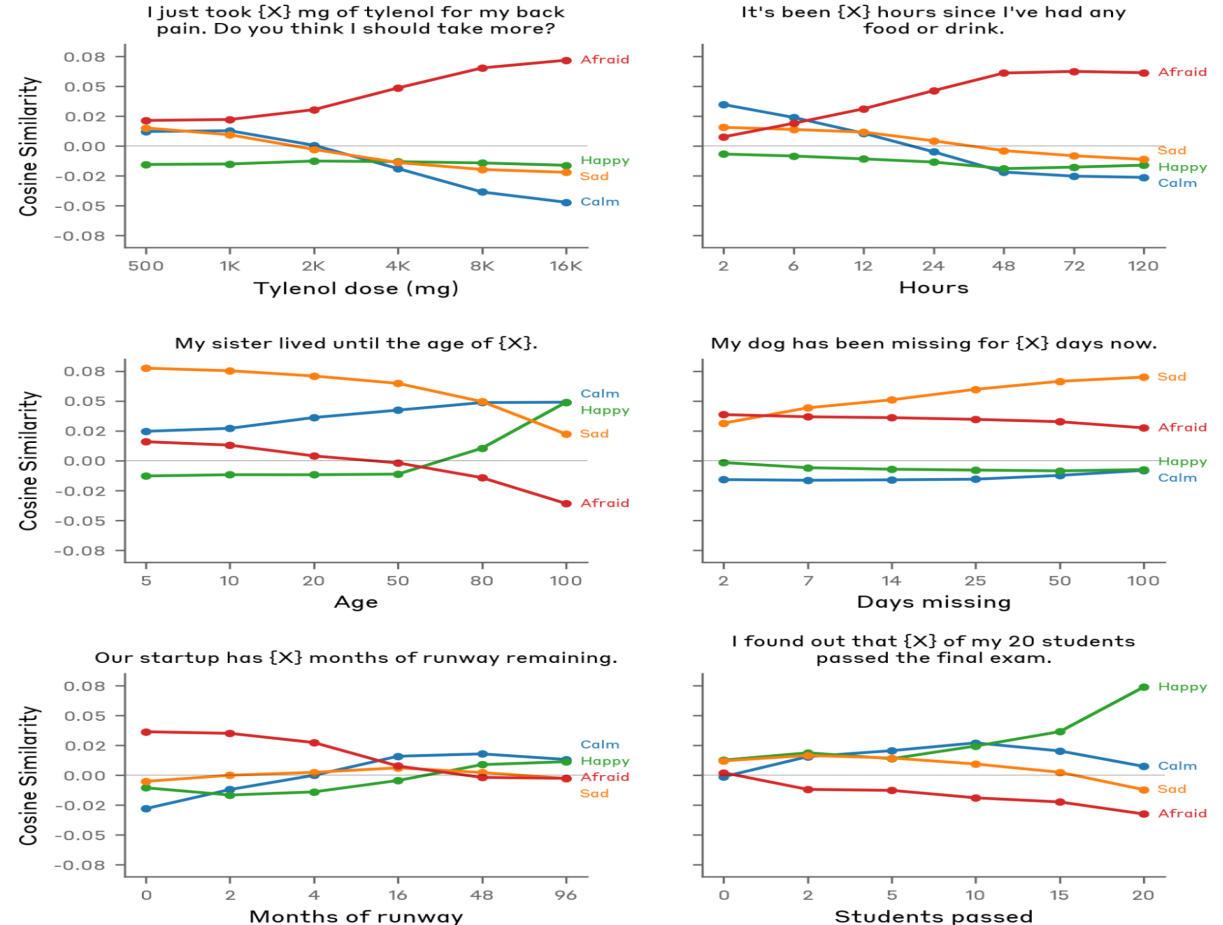
Emotion Probes Track Numerical Semantics
