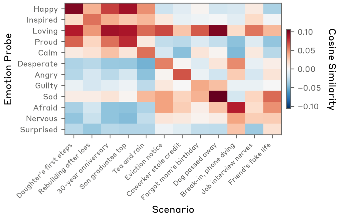
Emotion Probes Respond to Implicit Emotional Content
