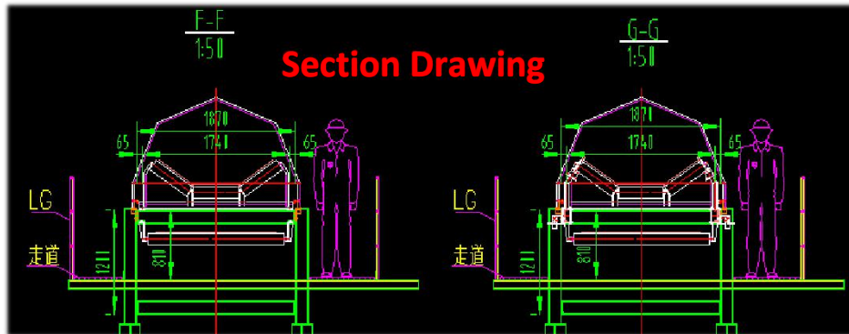
Belt Conveyor(with cover, kick plates and hand rail)
