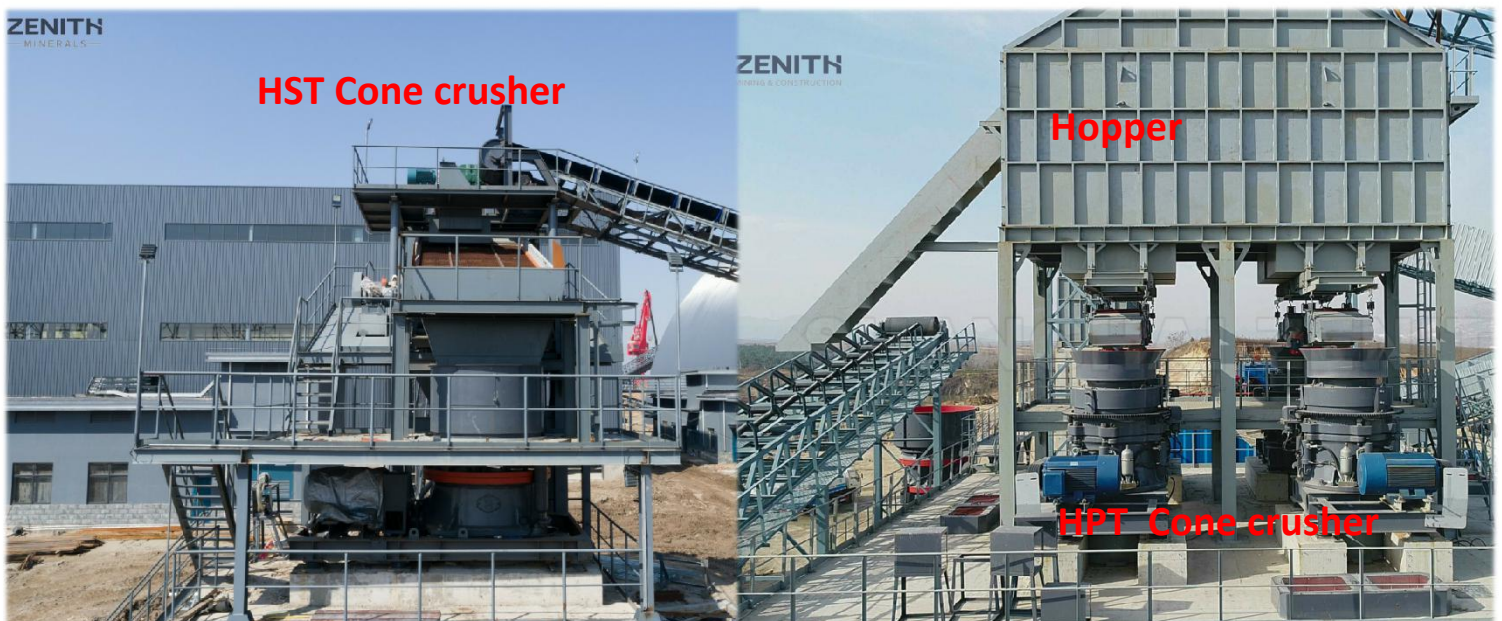
Cone Crusher(Steel Structure With hopper)
