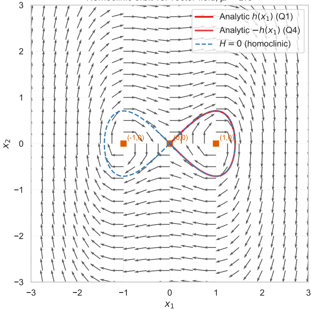
Homoclinic orbit vs. vector field, \mu = 1.0
