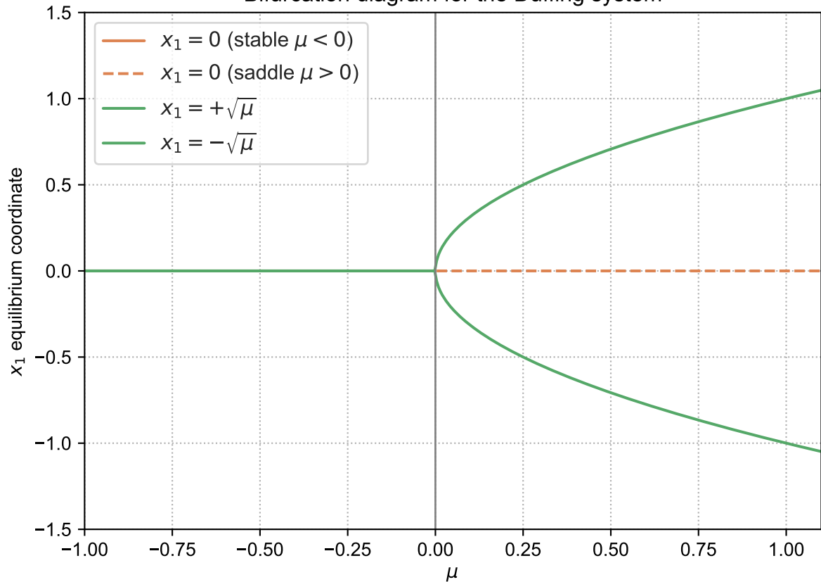
Bifurcation diagram for the Duffing system
