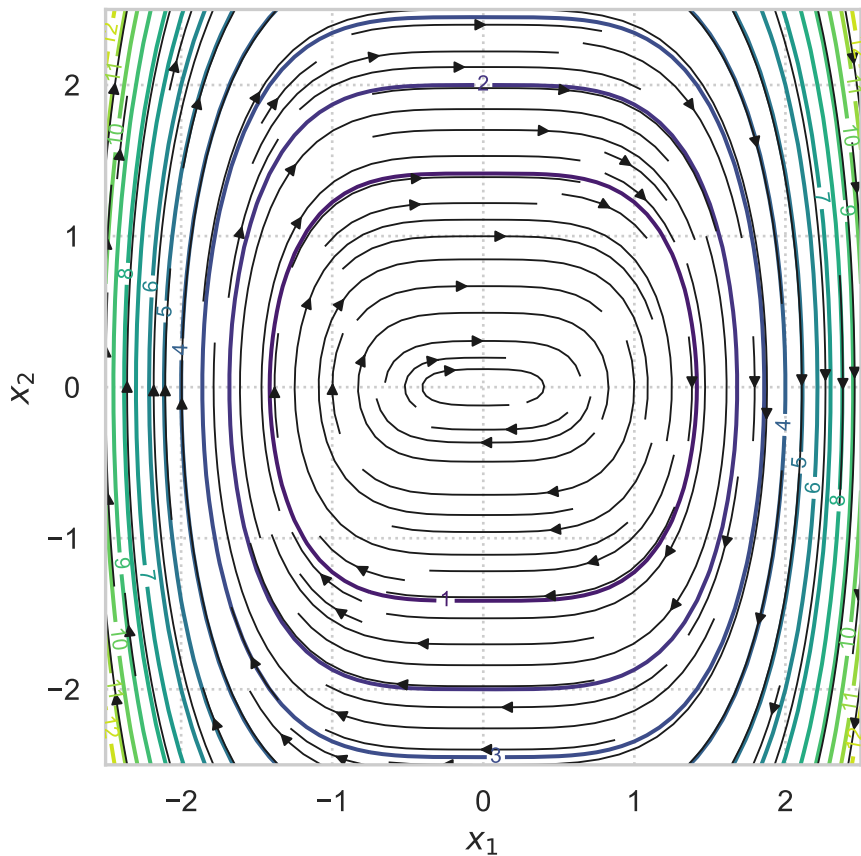
Vector field vs. level sets of V for \mu = 0
