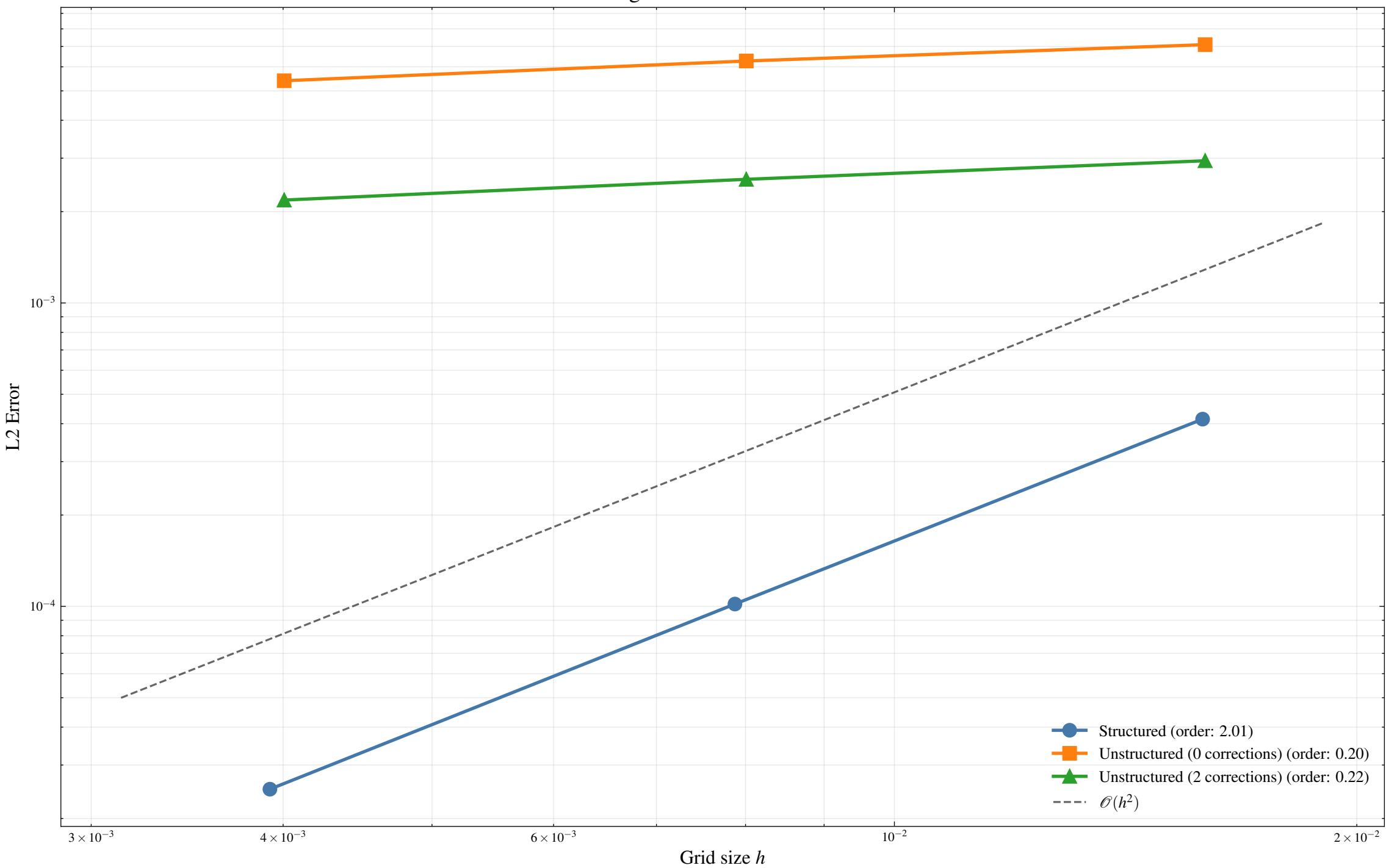
Order of Accuracy: Pressure Poisson Equation Effect of Non-Orthogonal Corrections on Unstructured Grids
