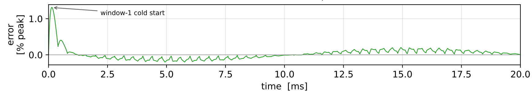
(c) co-sim – monolithic interface current: RMS 0.19 %, max 1.31 % of peak (at the window-1 cold start)
