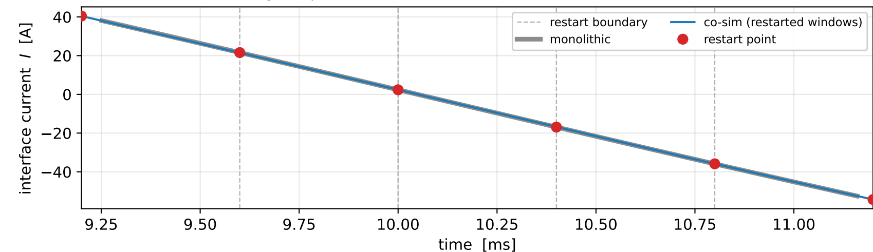
(c) co-sim – monolithic interface current: RMS 0.19 %, max 1.31 % of peak (at the window-1 cold start)
