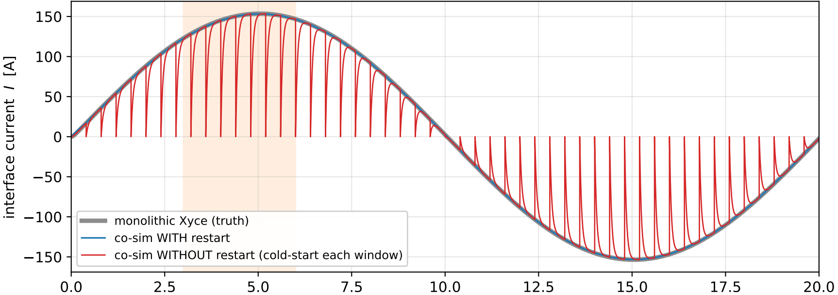
(b) zoom: without restart the inductor current resets to 0 each window (sawtooth); with restart it is continuous
