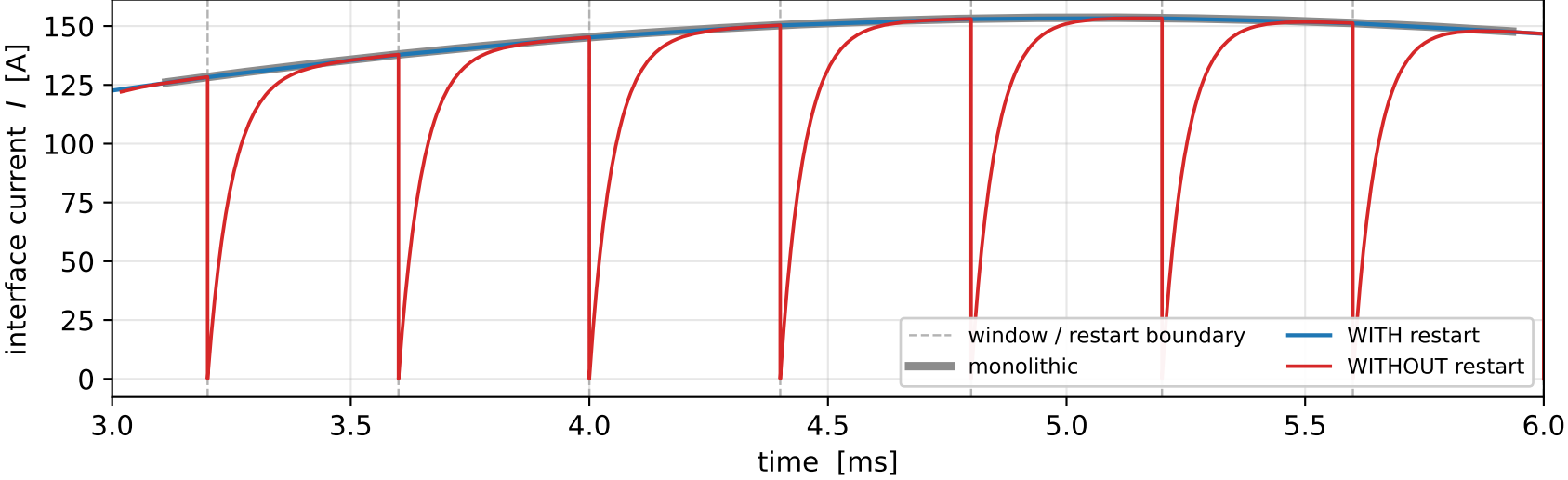
(b) zoom: without restart the inductor current resets to 0 each window (sawtooth); with restart it is continuous
