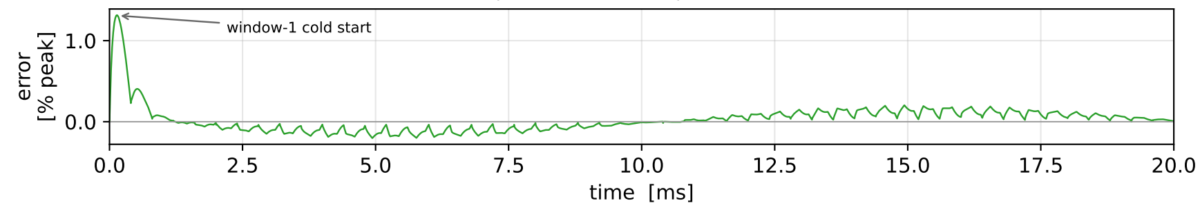
(c) co-sim - monolithic — RMS at restart points = 0.047 % of peak
