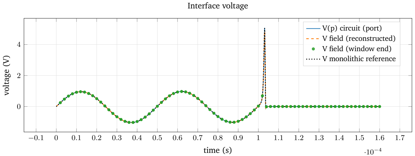
Figure A.1: Plot of the converged interface voltage of the third preset at 100 windows using the backward EULER discretisation and a voltage-driven field. The other parameters are the same as in Figure ??
