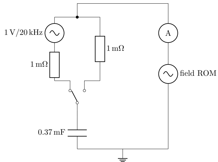
Figure 5.5: Circuit schematic of the fourth preset. The RLC circuit is being driven by a 1 V/20 kHz source. Switching commutates the loop from the source branch to a 1 m \Omega . Here depicted with the accumulated interface.
