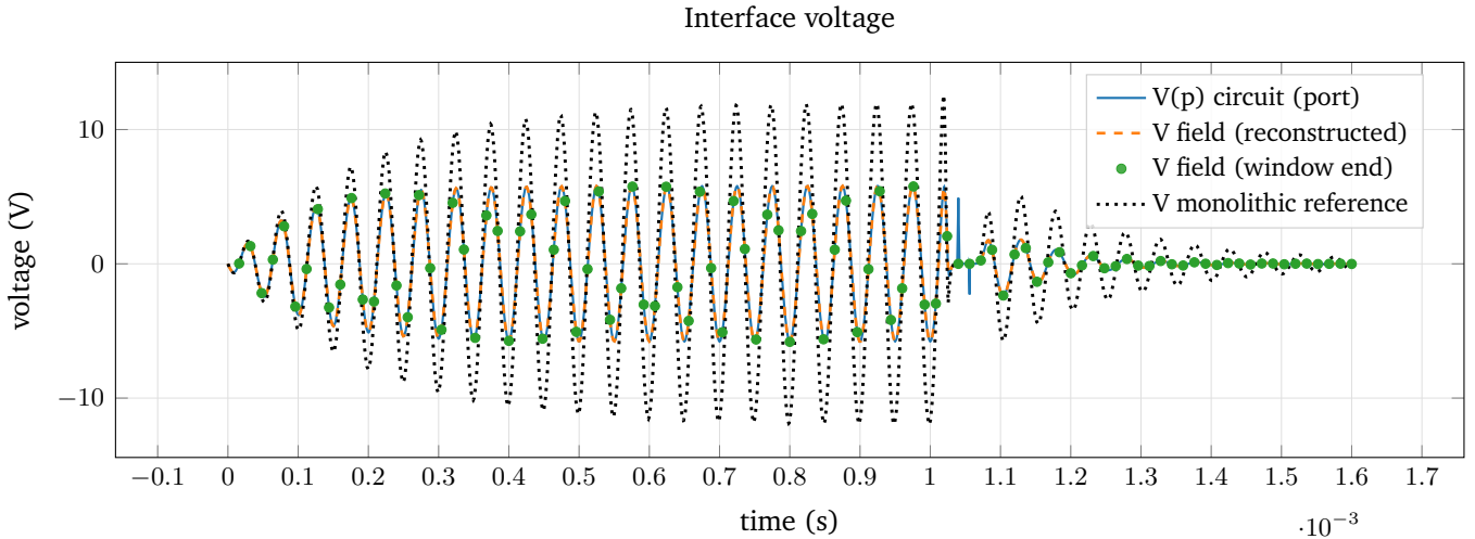
Figure A.2: Plot of the converged interface voltage of the fourth preset using the accumulated discretisation of the interface. 10 field evaluations and 200 circuit samples per window. The other parameters are the same as in Figure ??.
