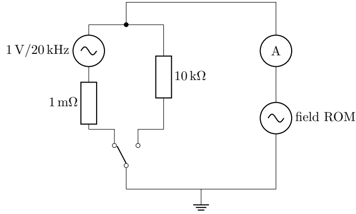
Figure 5.3: Circuit schematic of the third preset. Here depicted with the accumulated interface. At the switching instant, the source branch is disconnected and the 10\text{ k}\Omega resistor is switched into the loop (RL freewheel).
