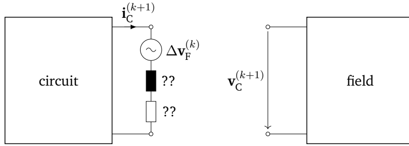
Figure 2.2: Schematic representation of the k + 1 -th Gauss–Seidel iteration for the field-circuit subsystems, using an approximation of the optimal transmission coupling condition.
