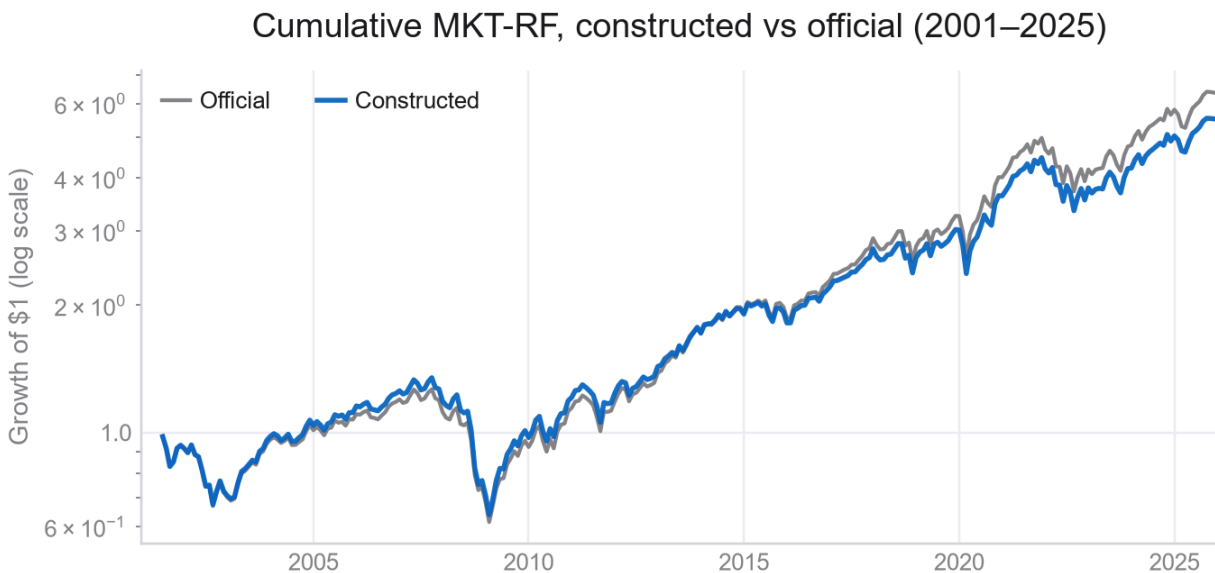
Cumulative MKT-RF: constructed vs official (2001–2025).
