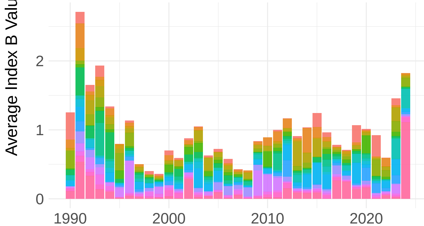
Instability of Regime
