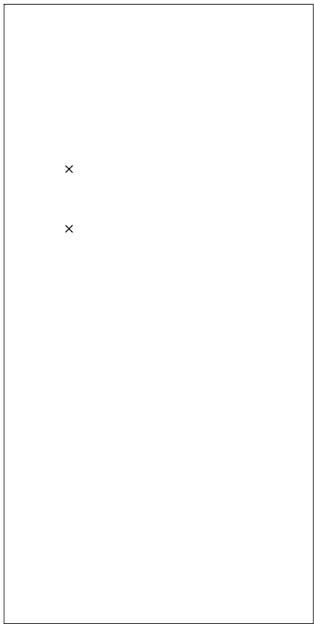
Drill Map: x 0.650mm / 0.0256" (2 holes) (not plated)
