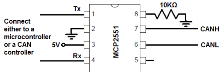
Figure 6 Transceiver MCP2551 wiring diagram
