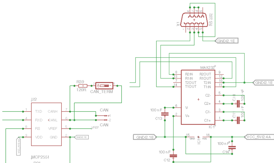
Figure 9 CAN and RS232 interface
