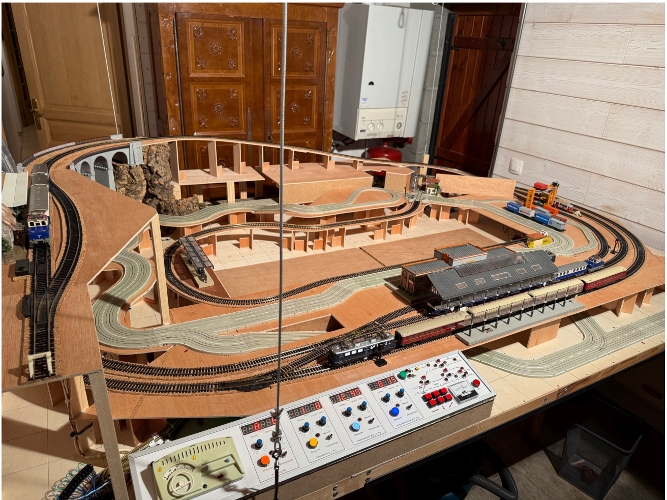
Figure 19 Railway network (31/07/2025)
