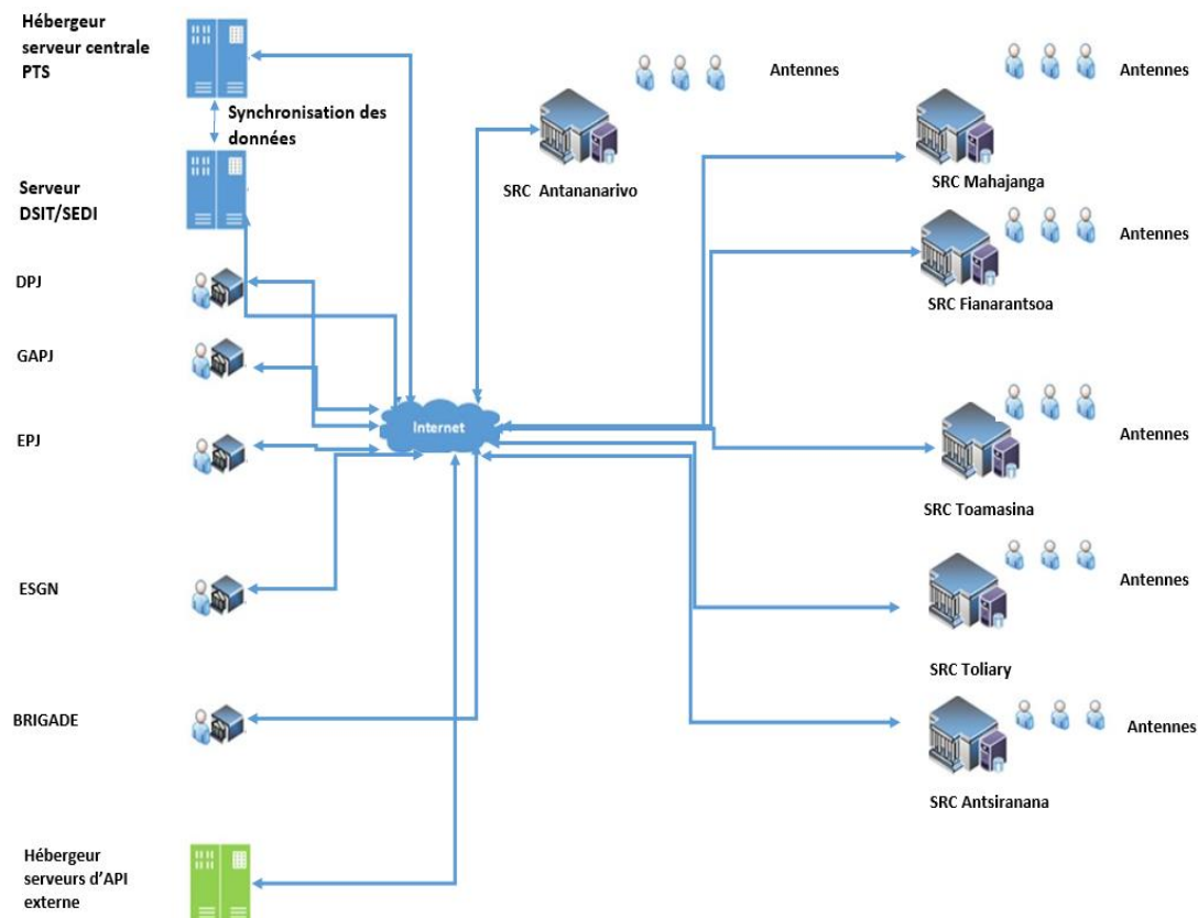
Figure 1 - Schémas architecture technique.
