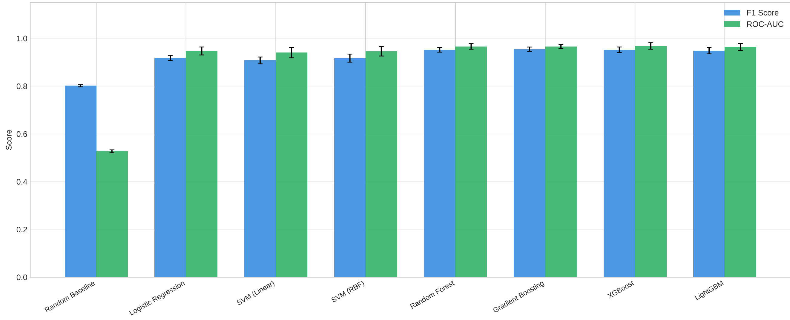
Multi-Classfier Comparison (All 26 Features, StratifiedGroupKFold)
