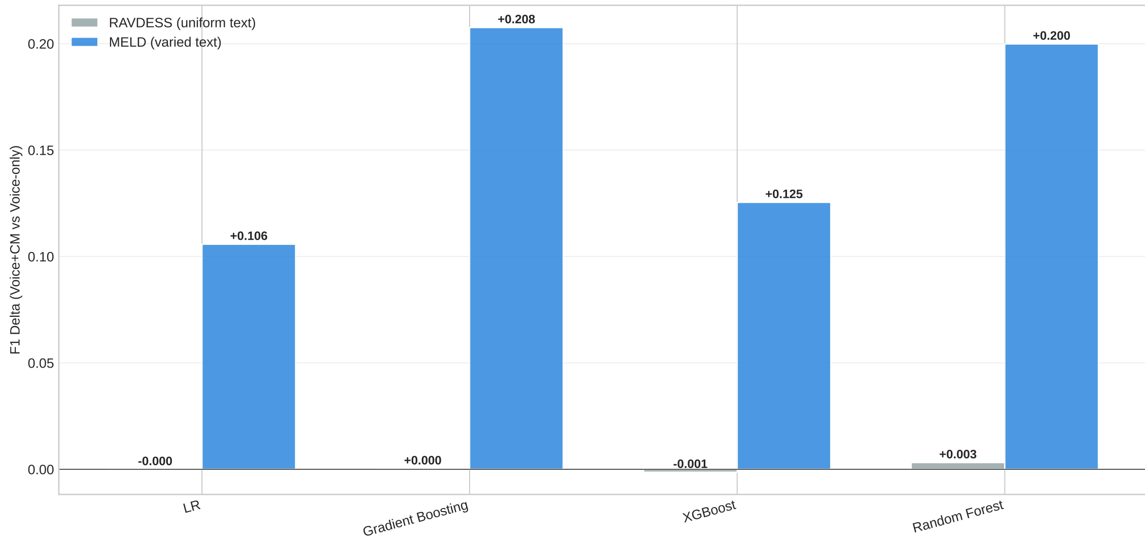
Cross-Modal Feature Contribution: RAVDESS vs MELD
